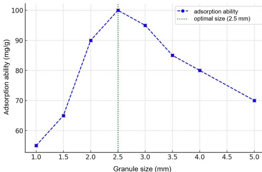
FIGURE 1. Effect of GCA Granule Size on Adsorption Capacity
