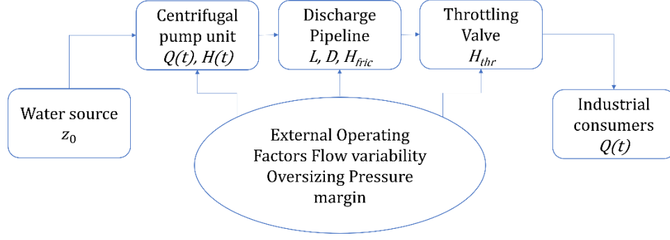
FIGURE 1. General Industrial Water Supply System
