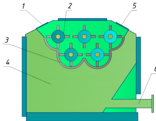
FIGURE 2. Five-drum shaking machine proposed by S.A. Noskova
