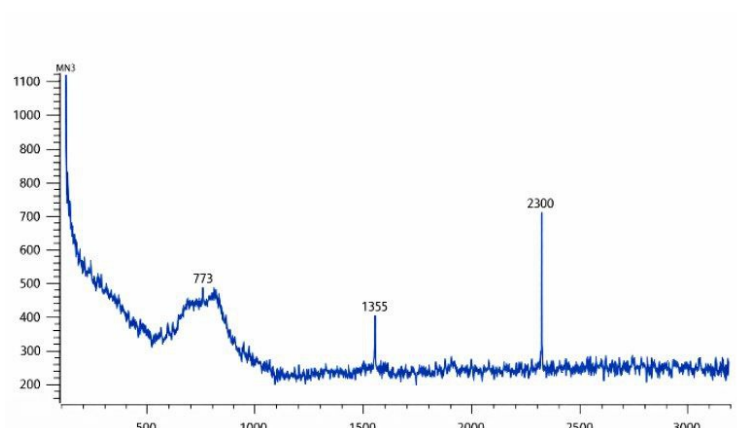
FIGURE 3. Rhenium metal sample Raman spectrum
