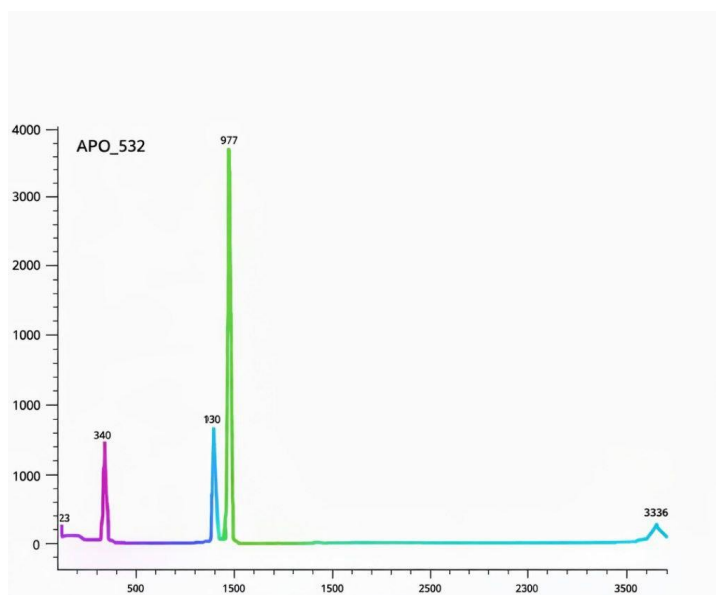
FIGURE 2. Ammonium perrenate Raman spectrum
