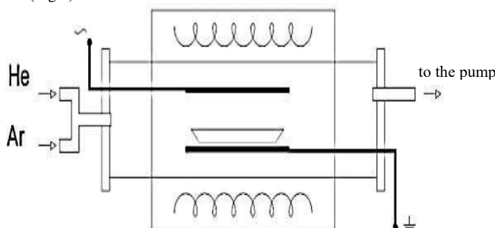
FIGURE 1. Principal diagram of a plasma chemical reactor
