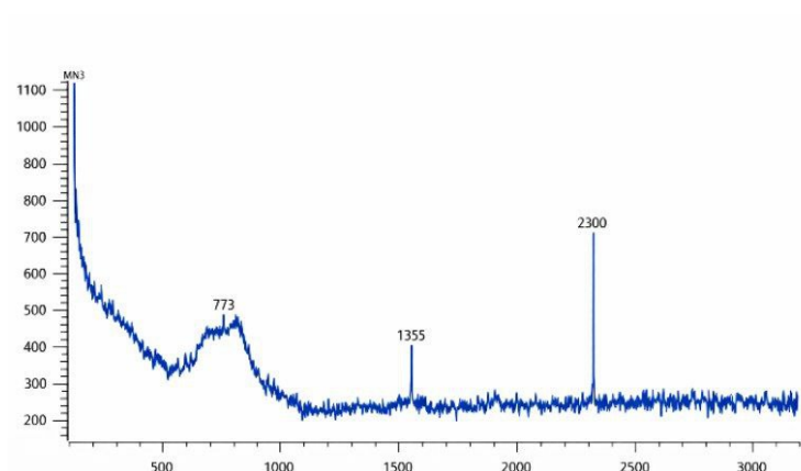
FIGURE 4. Rhenium metal sample Raman spectrum
