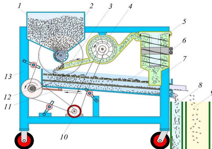
FIGURE 1. Technological scheme of safflower seed cleaning machine. 1–bunker; 2–supply roller; 3– suction pipe; 4–fan; 5–dust sinking device; 6–upper sieve; 7–lower sieve; 8–container with foreign admixtures; 9–clean seed container; 10–electric motor; 11–a connecting rod that moves the sieve; 12–oscillating device; 13–machine framework.
