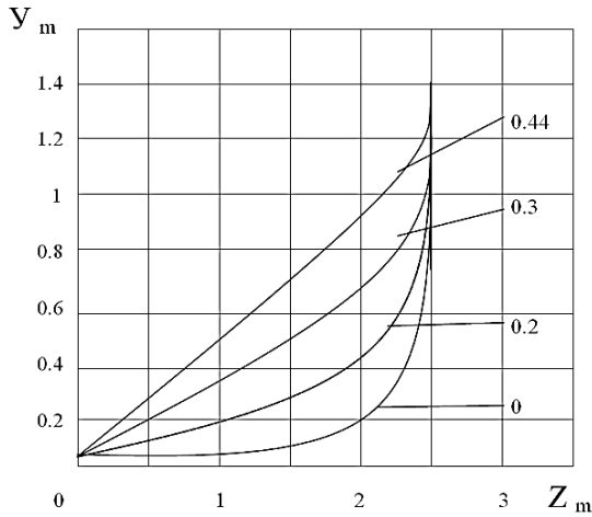
FIGURE 2. Regulation characteristics for a resistive (active) load
