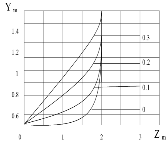
FIGURE 3. Regulation characteristics for a resistive–inductive load
