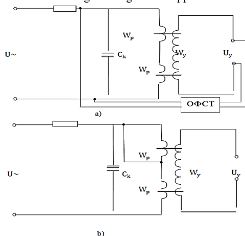
FIGURE 1. Circuit configurations of a ferromagnetic current stabilizer
