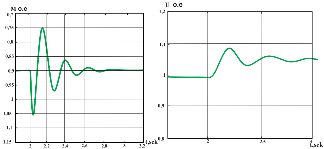
FIGURE 3. Changing torque and voltage synchronous
