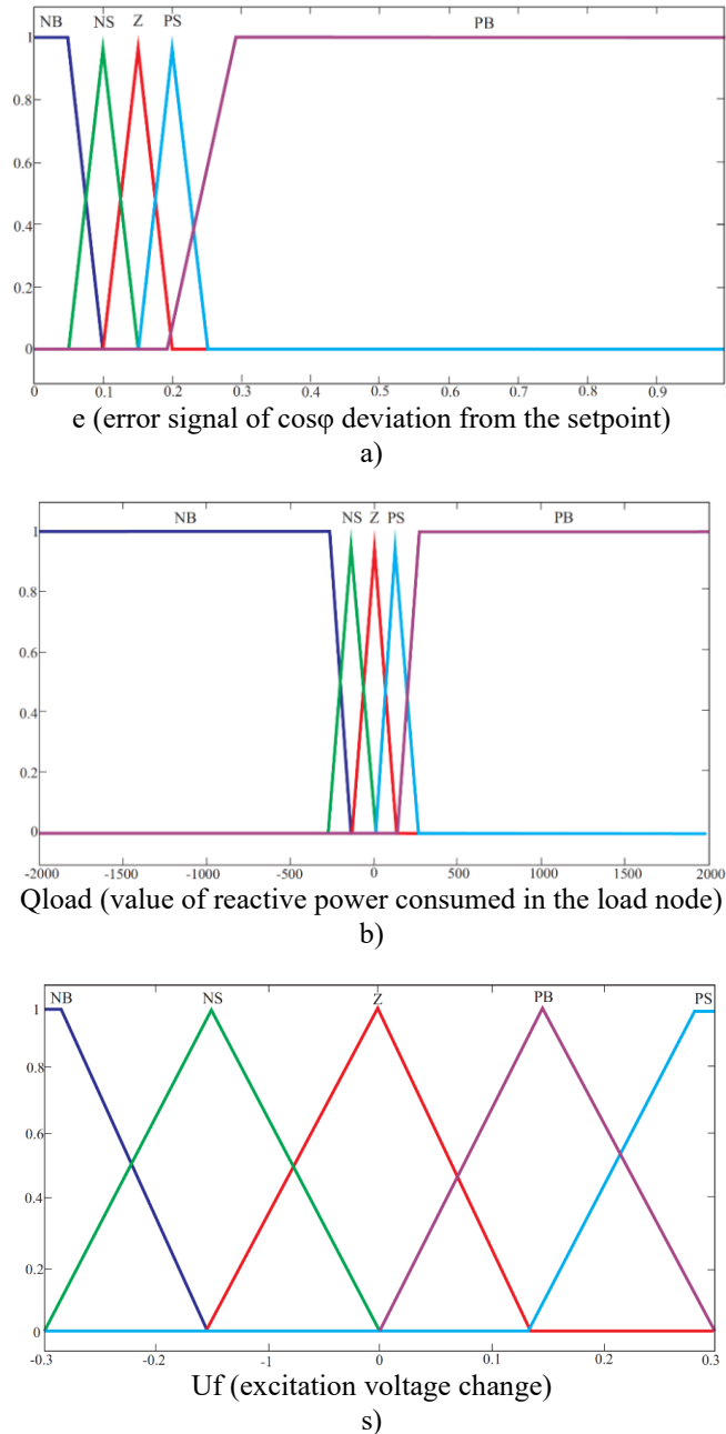
Fig. 1. Membership functions of input and output parameters
