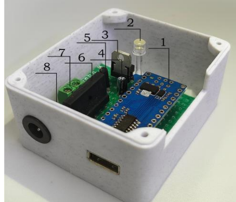
FIGURE 2. Internal structure of the EHRK-2024 device
