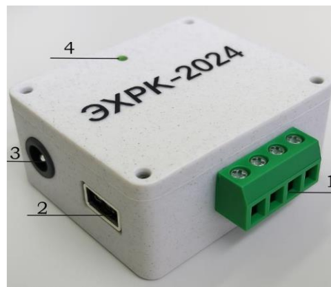
FIGURE 1. External view of the EHRK-2024 device
