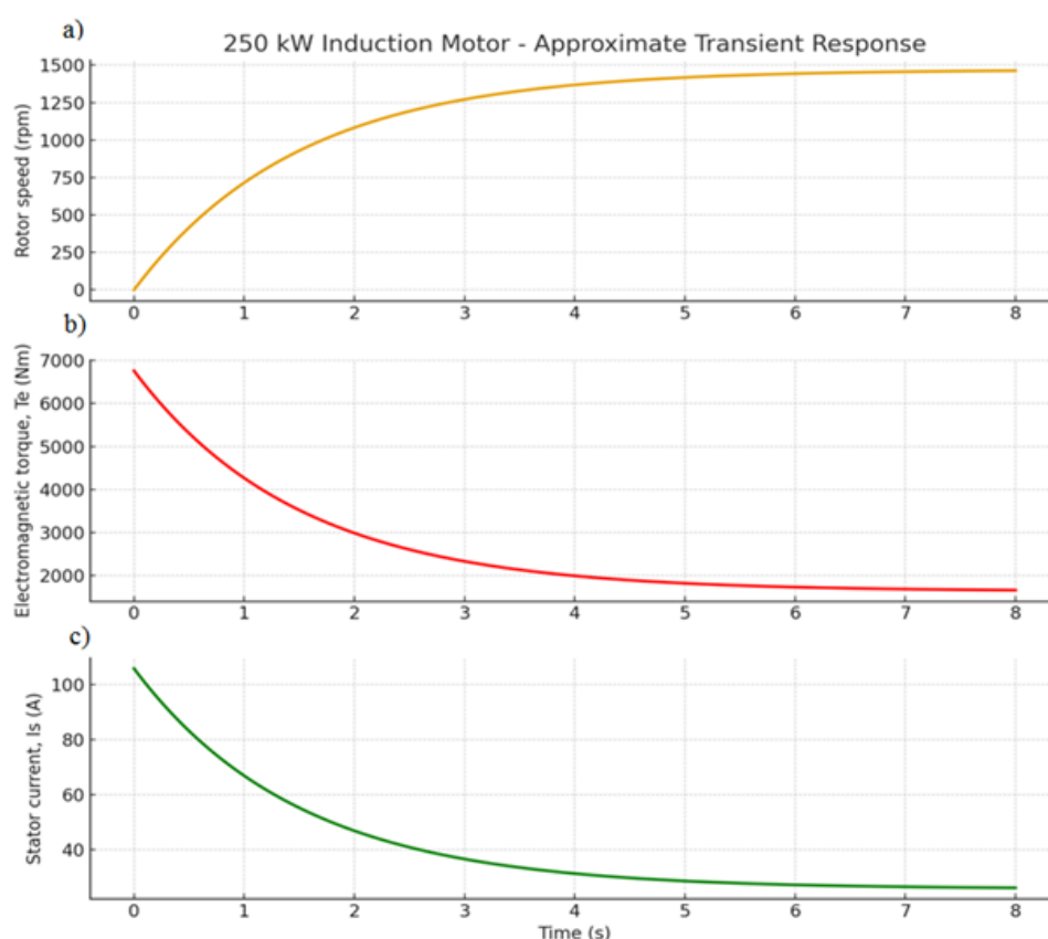
FIGURE.4. Mechanical characteristic of an asynchronous motor with a fan power of 250 kW.
