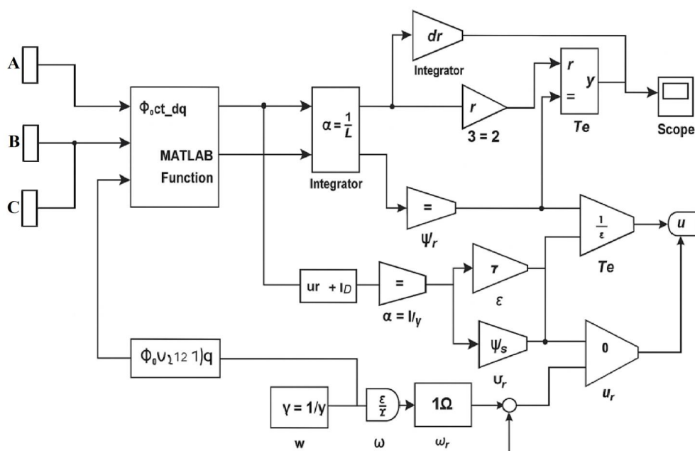
FIGURE 1. Algorithm of asynchronous motor dynamics in a Simulink environment
