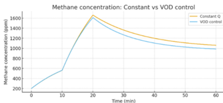
FIGURE.2. Change in methane concentration over time (comparison of constant ventilation and VOD regime)
