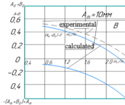
Fig. 3. Dependence of A_0 , B_0 , and A_0 + B_0 = f(m_1/m) of a single-stroke EMVD with bias magnetization
