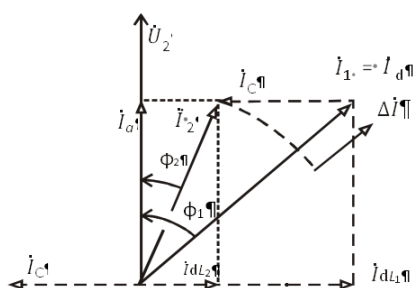
FIGURE 2. Vector diagram of cross-capacitive compensation in a circuit
