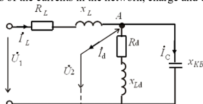
FIGURE 1. Transverse capacitance compensation replacement scheme
