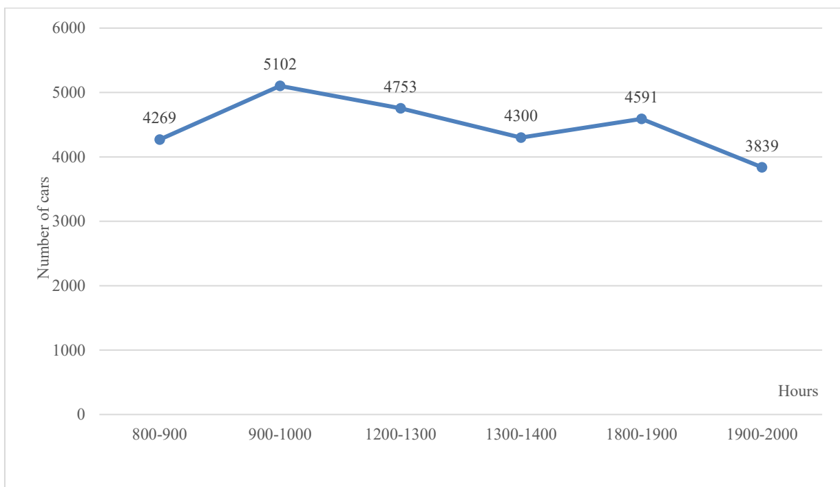
FIGURE 2. Graph showing variations in traffic flow by hourly intervals at the Karakalpakstan–Gubar Street intersection in Uzbekistan.
