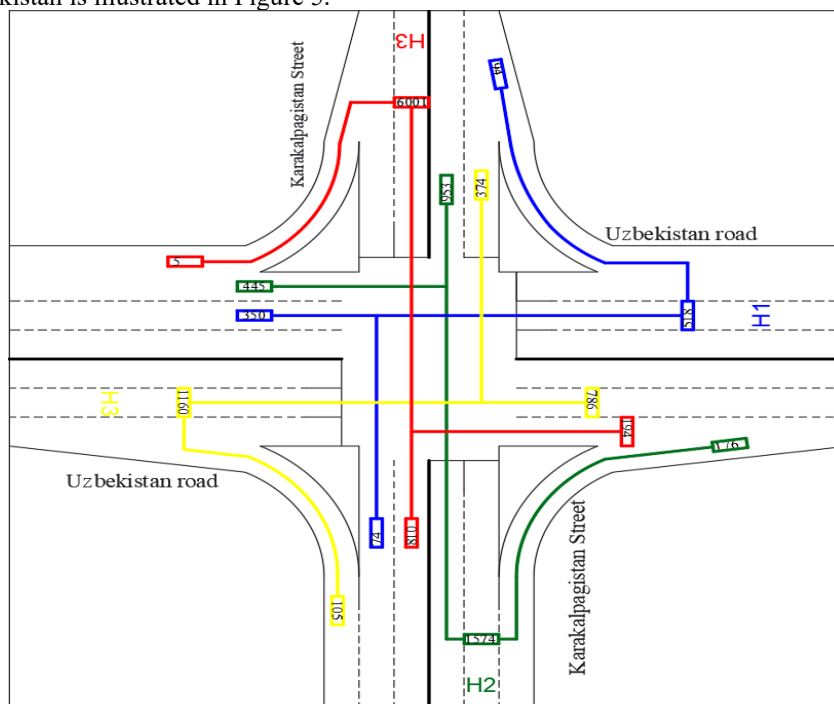
FIGURE 4. Conditional cartogram illustrating the intensity of traffic flows at the intersection of Karakalpakstan Street and the Uzbekistan road.
