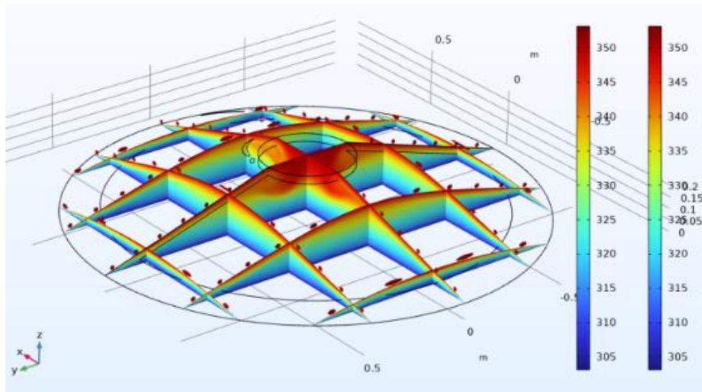
FIGURE 3. Changes in heat distribution in the working chamber of a simple solar water heater with a reflector and a tubular system at different points in time.
