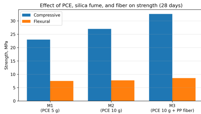
FIGURE 3. Effect of PCE dosage, silica fume, and polypropylene fiber on strength (28 days).
