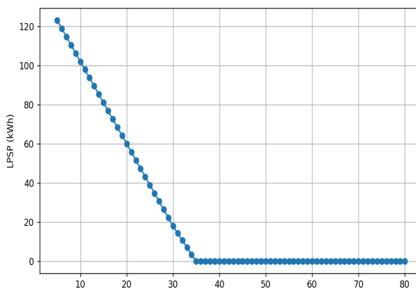
FIGURE 3. Insufficient energy compared to battery capacity
