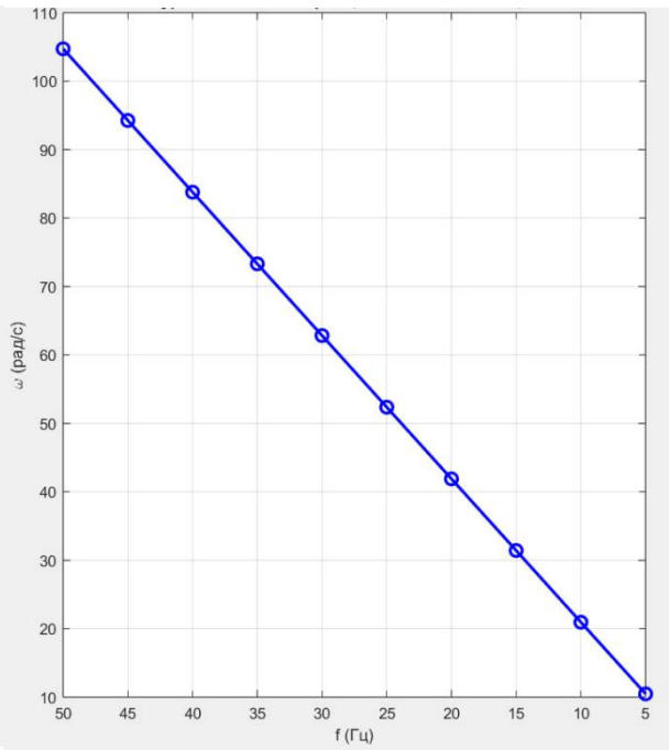
FIGURE 3.c. Graph of the dependence of the angular velocities of the frequency-controlled asynchronous electric drive of the feeder device on the network frequencies according to the control law U1/f1=\text{const}
