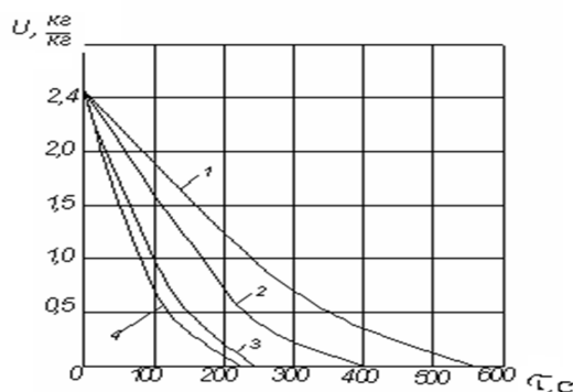
FIGURE 5. Drying curves for 280 g/m 2 cellulose in a conductive dryer
