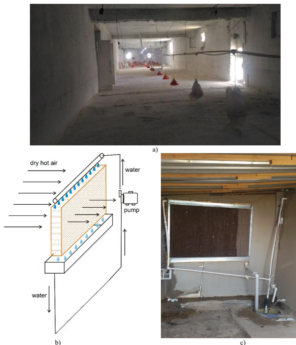
FIGURE 1. Poultry farm "Zhumabozor" in Tashkent region (a), operating principle (b), and design of the evaporative cooling system (c)
