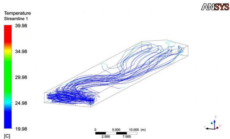
FIGURE 5. Air current patterns in the poultry house
