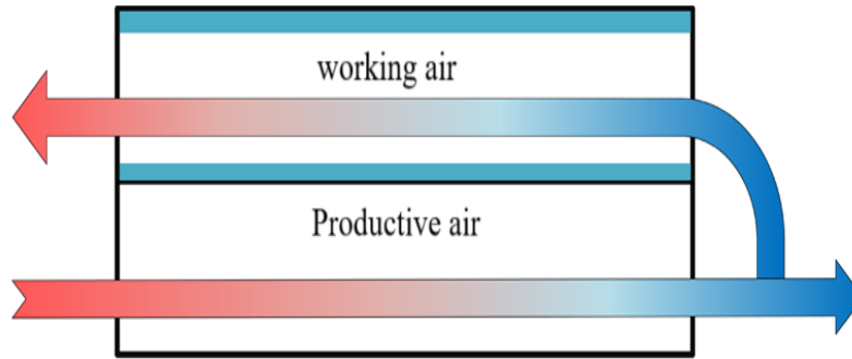
FIGURE 2. Regenerative indirect evaporative cooling
