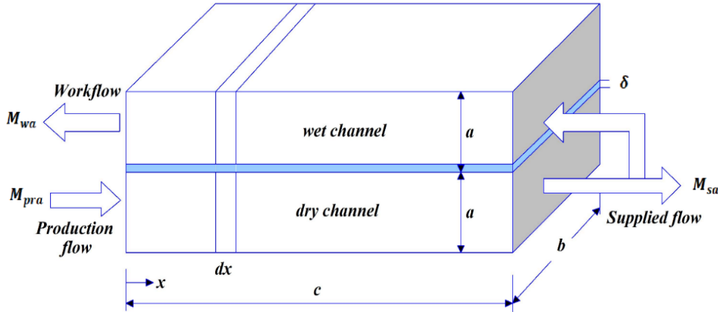
FIGURE 3. The scheme of the regenerative heat and mass transfer apparatus
