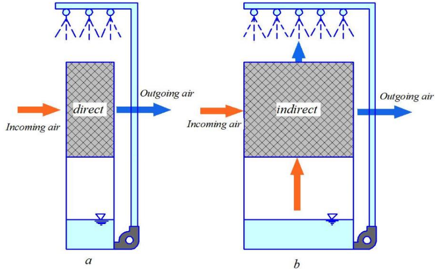
FIGURE 1. Types of air evaporative cooling
