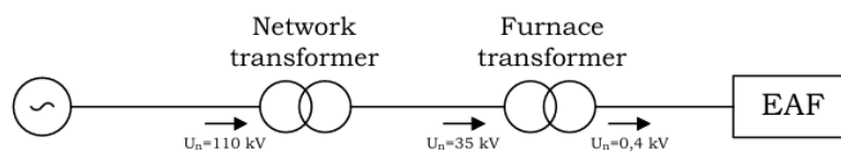
Fig. 1. Electrical supply diagram for electric arc furnaces
