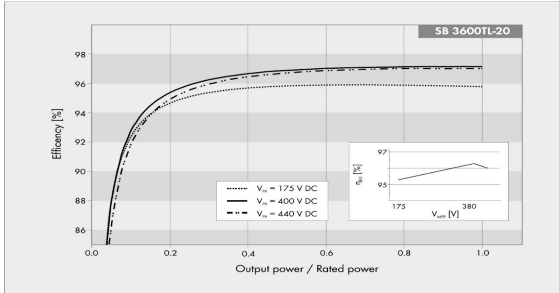
FIGURE 5. Inverter Performance Based on Solar Cell Load
