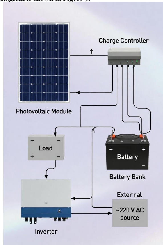
FIGURE 6. Inverter wiring diagram
