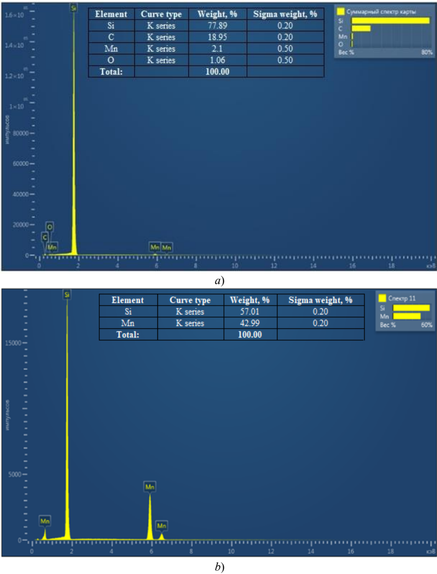
Fig. 1. Elemental analysis of silicon samples obtained by electrodiffusion: a) - “positive” sample, b) - “negative” sample.
