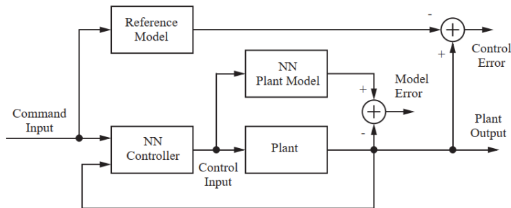
FIGURE 3. Control system rooted in reference model.
