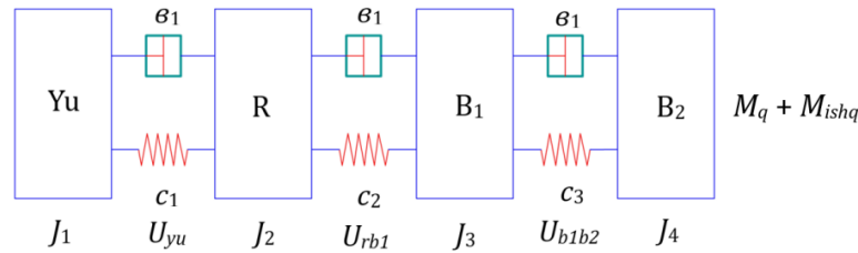
1-mass, rotor of the electric drive; 2-mass, the masses of the rotating elements of the reducer brought to the output shaft and the mass of the half-coupling; 3-mass, the mass of the half-coupling and the driving drum; 4-mass, the mass of the driven drum is taken
