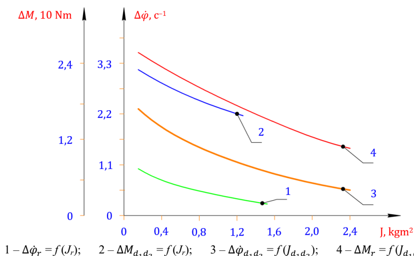
FIGURE 7. Graphs of the dependence of the angular velocities and turning moments of the roller mechanisms with a bearing support with a belt element and a shaft of the leading and driven drums of the belt conveyor machine units on the force of change of their moments of inertia
