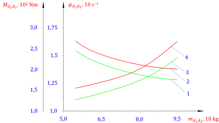
FIGURE 5. Graphs of the dependence of the angular velocity and loading of the leading and driven drums of the belt conveyor machine unit on the mass of gold ore (performance)
