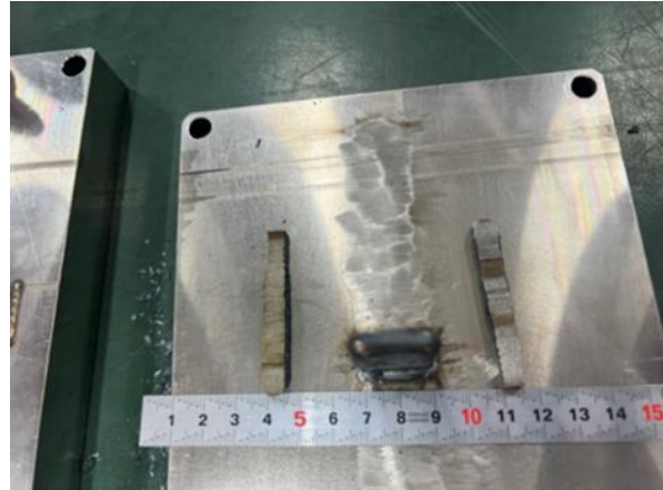
FIGURE 4. Samples for hardness testing
