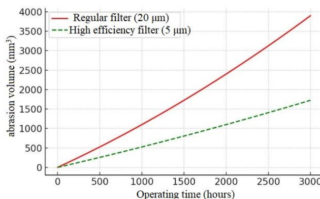
FIGURE 1. Effect of filtration efficiency on corrosion
