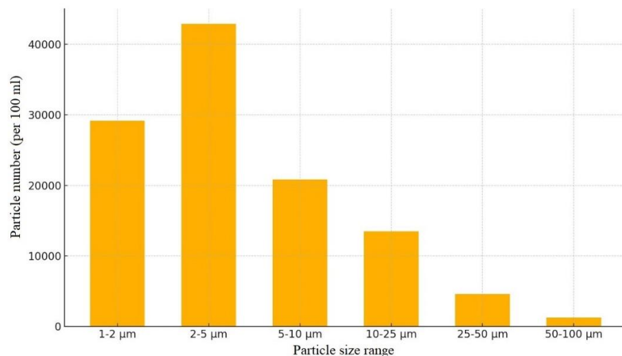
FIGURE 5. Particle content in pure hydraulic oil (average/10ml)
