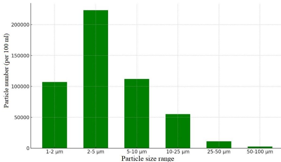
FIGURE 7. 1 - amount of particles in the filtered hydraulic oil (average/10ml)
