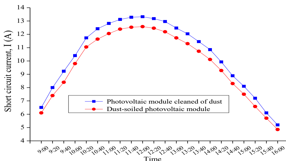
FIGURE 4. Time dependence of the short-circuit of a BPV module during the day
