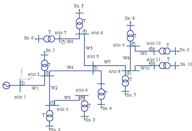
FIGURE 1. Electrical network diagram
