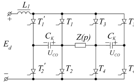
FIGURE 4. Single-phase ACI circuit with CT
