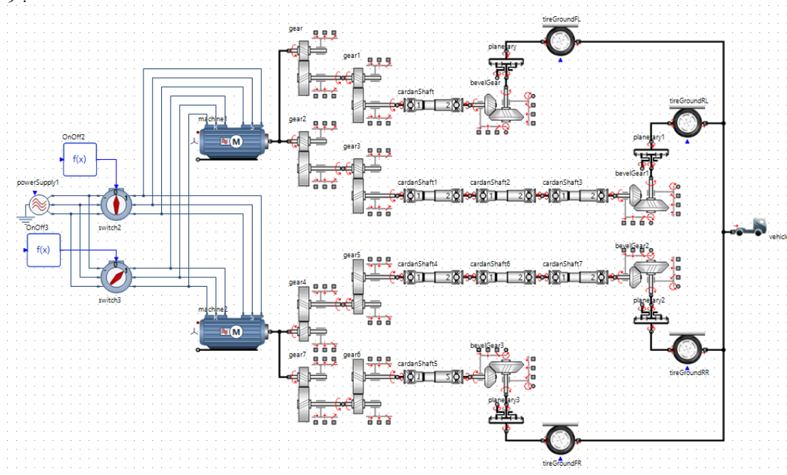
FIGURE 1. Simulation model of the MSPC kinematic scheme
