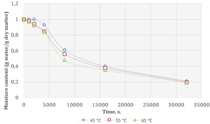
FIGURE 3. Changes in moisture content with time at different drying temperatures
