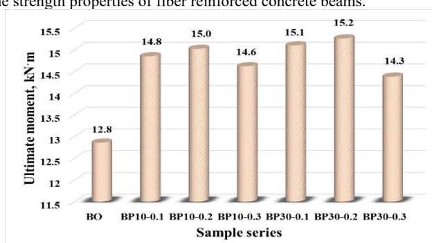
FIGURE 5. Strength characteristics of fiber-reinforced concrete beams
