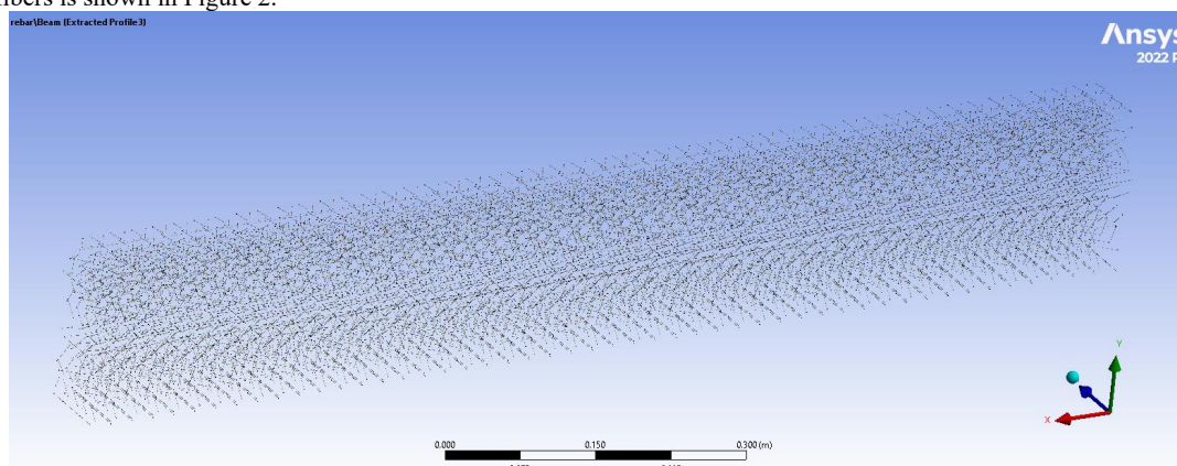
FIGURE 2. General view of modeled polypropylene fibers
