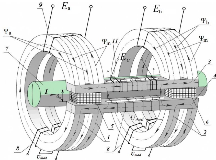
Figure 2. Simplified structural diagram of the current transducer
