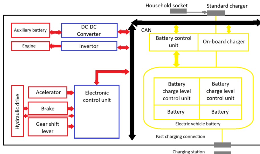
FIGURE 1. General block diagram of electric vehicle control
