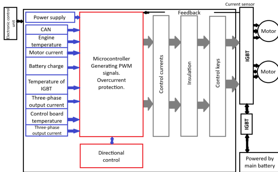
FIGURE 2. Block diagram of inverter control in electric vehicles
