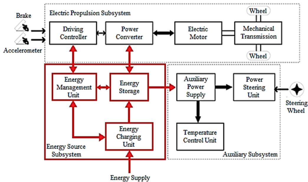
FIGURE 3. Subsystems of EVs
