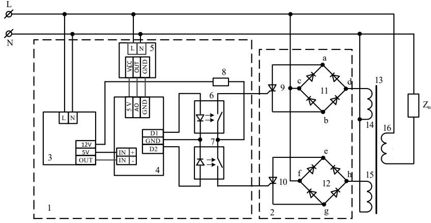
FIGURE 5. Automatic voltage sag restoration scheme
