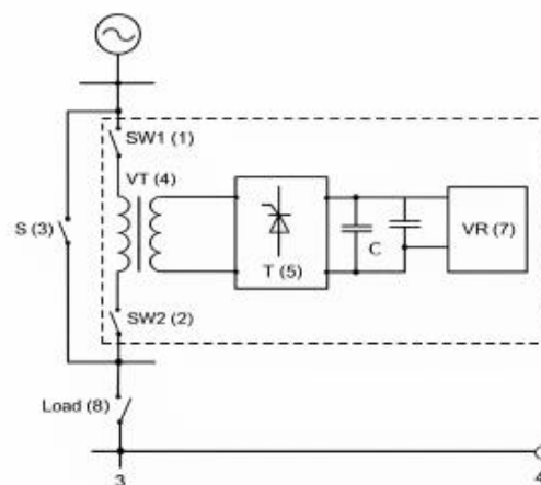
FIGURE 3. Dynamic voltage sag restoration device
