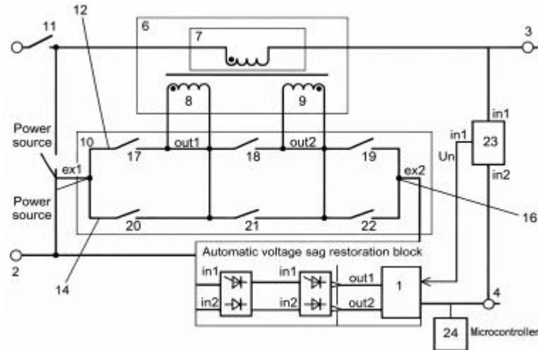
FIGURE 2. Schematic diagram of the alternating voltage regulator device
