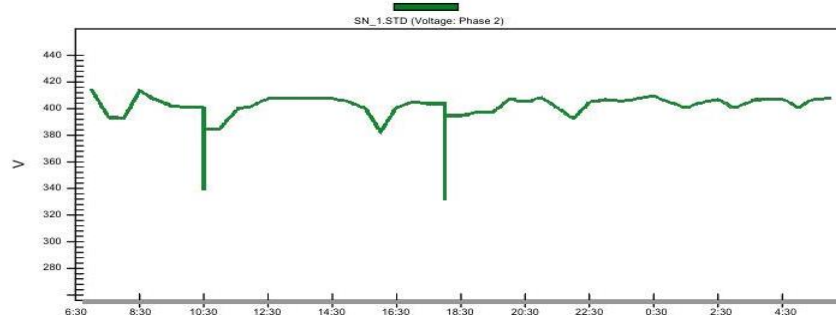
FIGURE 1. The voltage variation condition in the electrical network of a spinning enterprise
