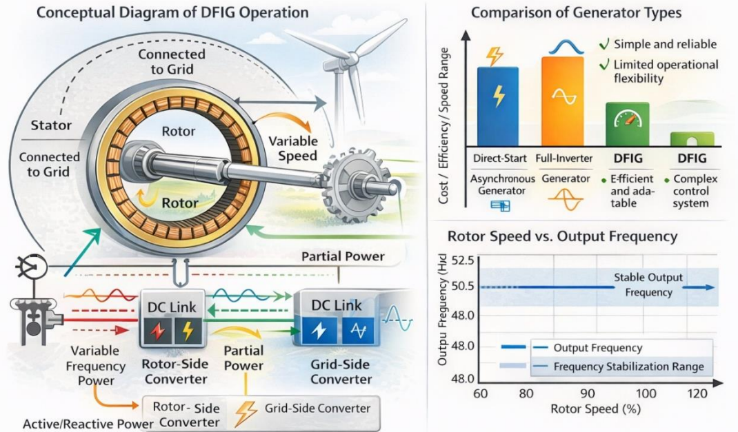
FIGURE 2. Composite diagram of DFIG operation, generator type comparison, and rotor speed versus output frequency
