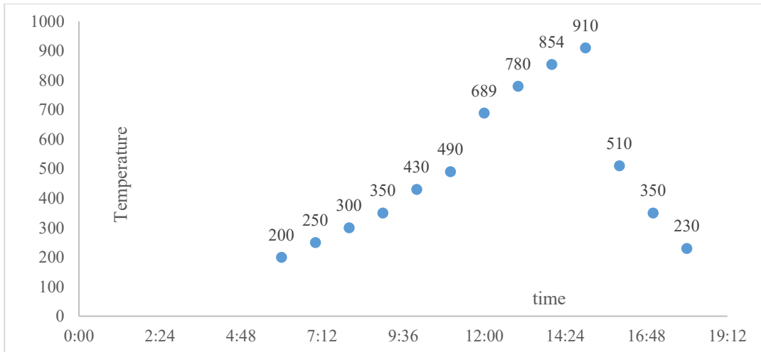
Figure 5. One-day results of a small-scale solar oven on a sunny day in March
