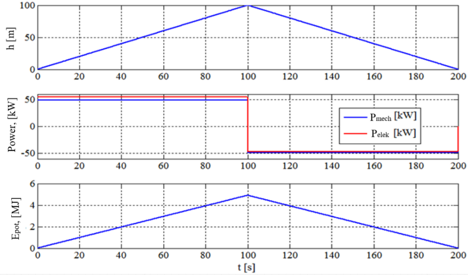
FIGURE 5. Model of the mass lifting (charging) and lowering (discharging) processes.
