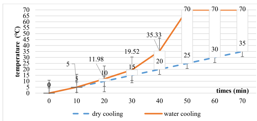
Figure 6. Liquid and dry air cooling
