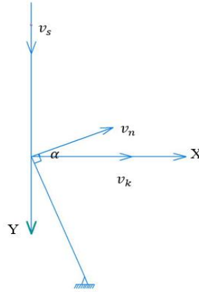
Figure 4. Direction of fluid velocities
