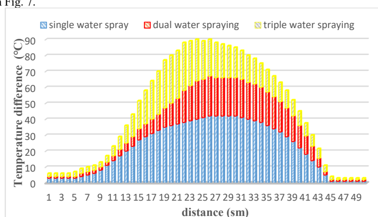
Figure 7. Difference in temperature and distance when the number of sprayers is different
