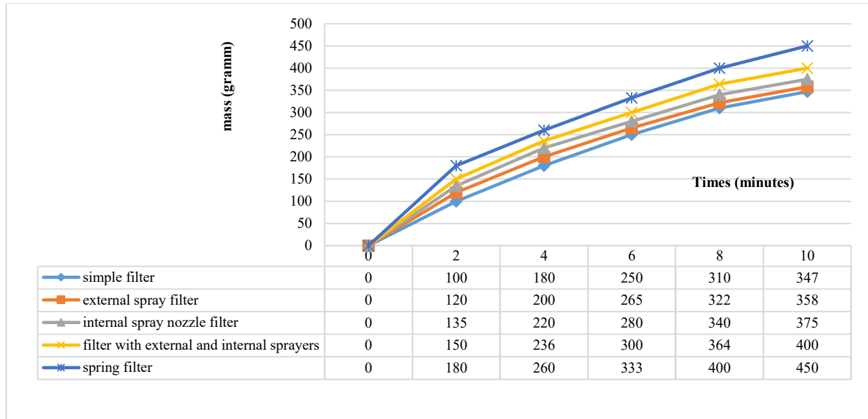
FIGURE 4. Graph of the time dependence of the amount of dust released from the filter
