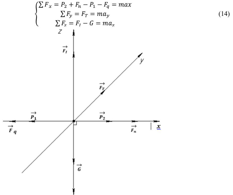
FIGURE 2. Directions of forces generated in the filter
