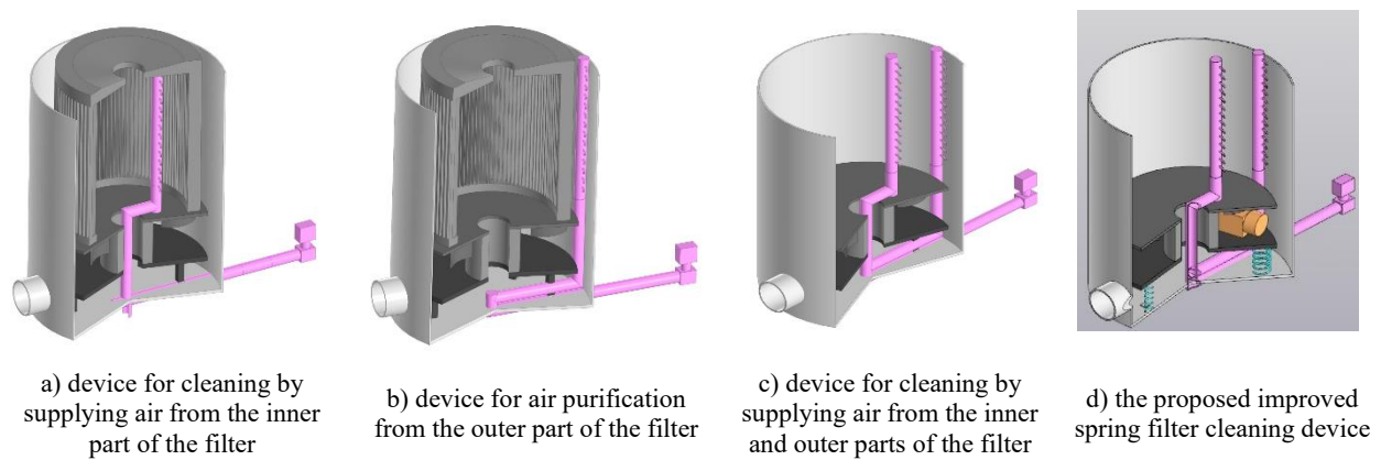
FIGURE 3. Existing and proposed filter cleaning devices
