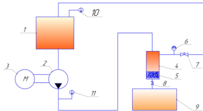
FIGURE 3. Schematic representation of the experimental setup
