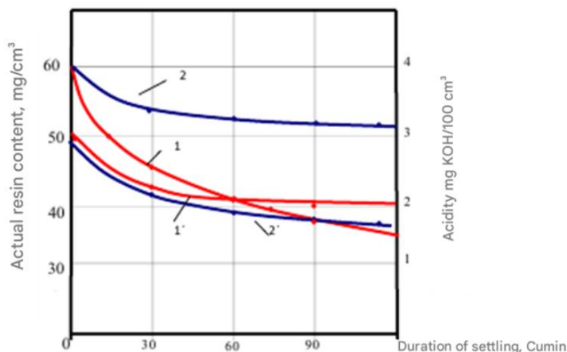
FIGURE 6. The dependence of the acidity and composition of the real resins in the fuel on the duration of the curd (Addition = 90 ° C) for different compounds
