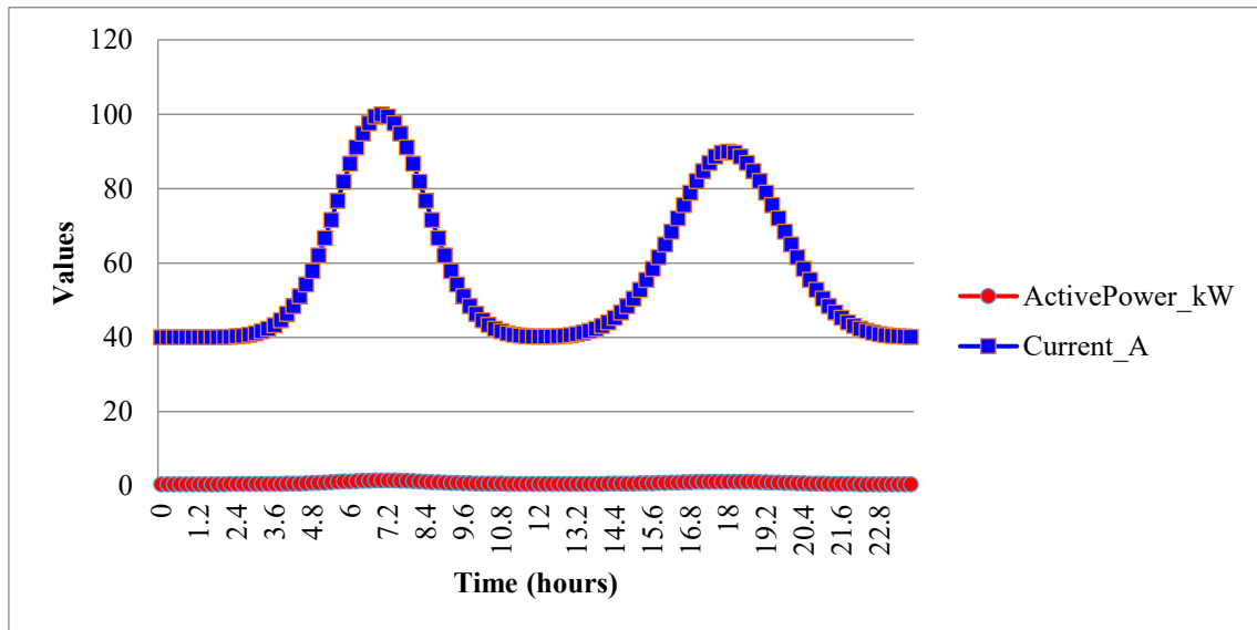
FIGURE 2. Active power and current relationship
