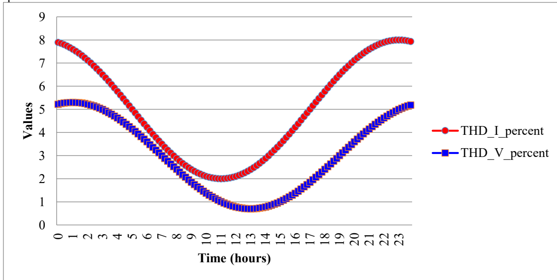
FIGURE 5. THD(I) & THD(U) distortion trends
