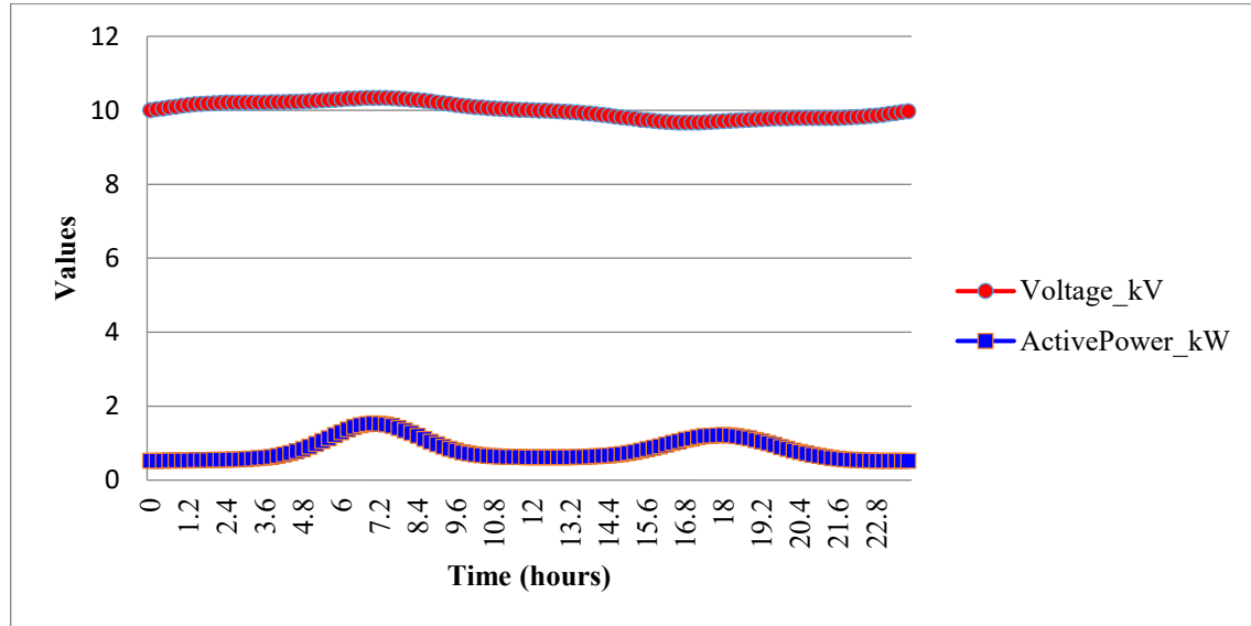
FIGURE 8. Voltage and active power correlation
