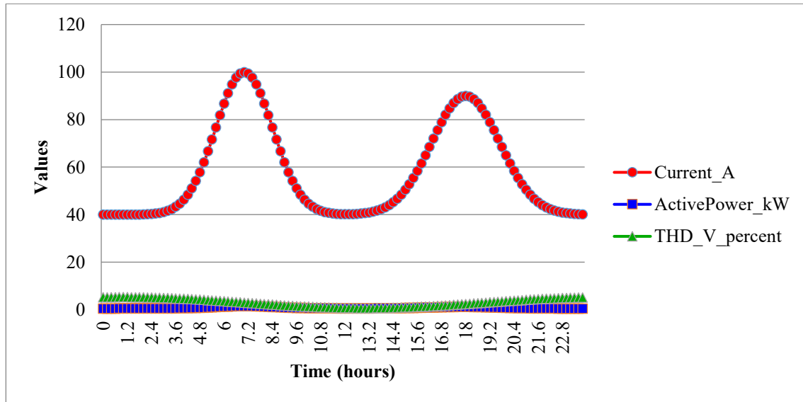
FIGURE 7. Current, power and distortion link
