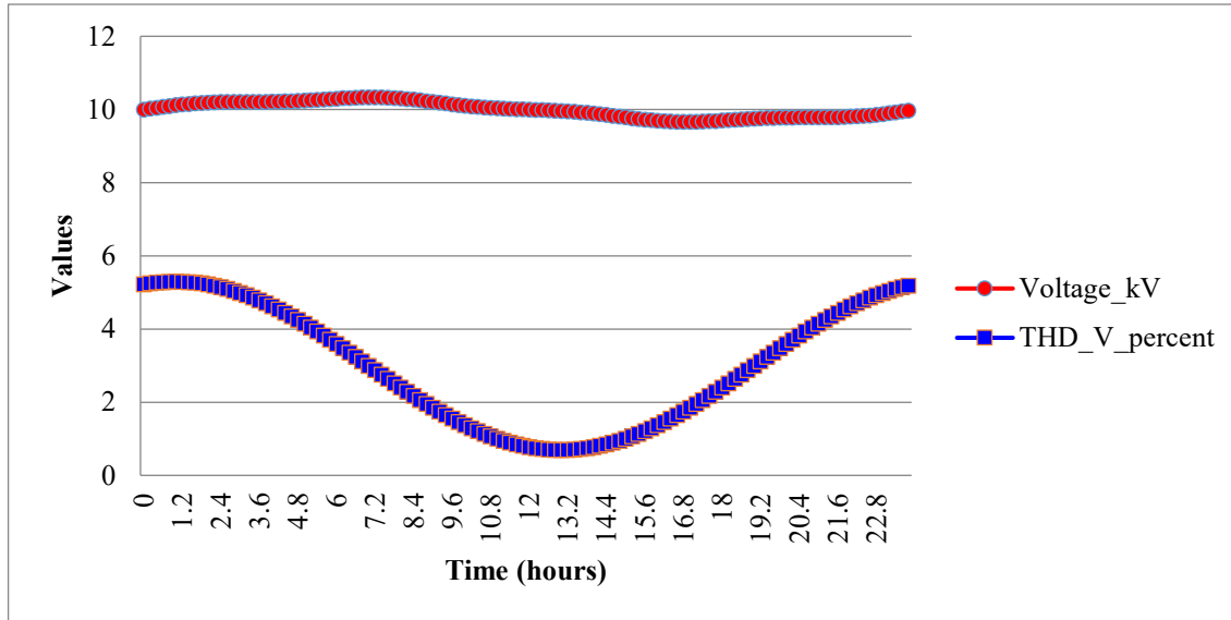
FIGURE 6. Voltage and THD(U) coupled behavior
