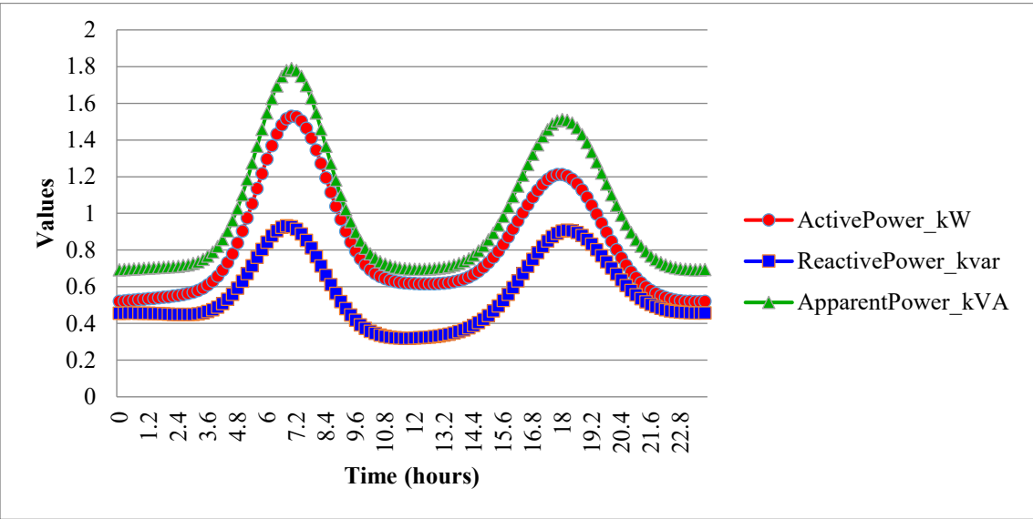
FIGURE 3. Power flow components over time
