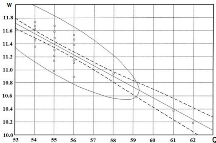
FIGURE 1. Correlation area and enrichment relationship \omega = f(Q_p)
