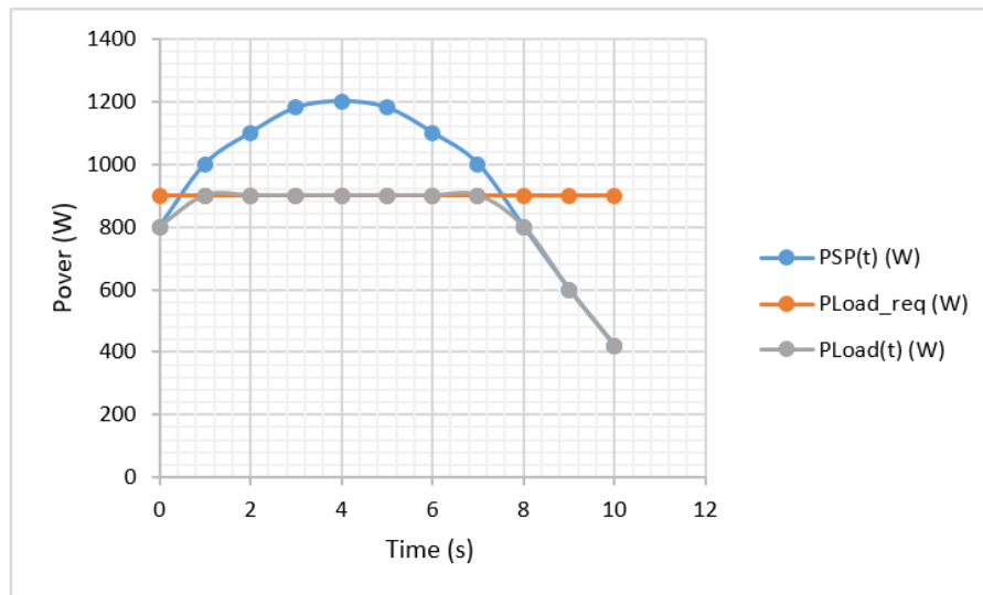
FIGURE 2. Time-dependent consumer load power.
