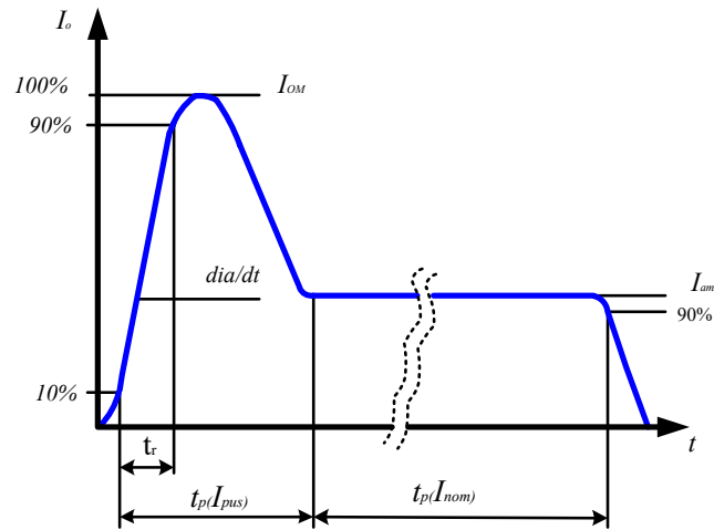
FIGURE 3. Time-dependent graph of the thyristor control pulse
