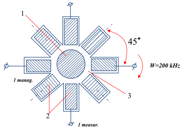
FIGURE 4. The principle of “rotating” the magnetic field:
