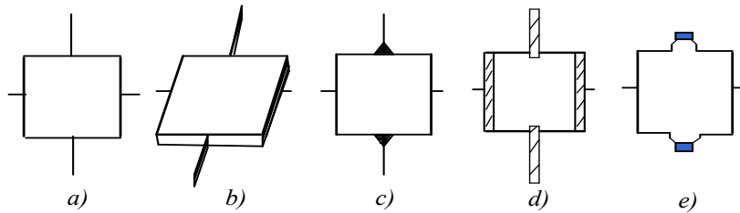
FIGURE 3. The shapes of Hall contacts:
