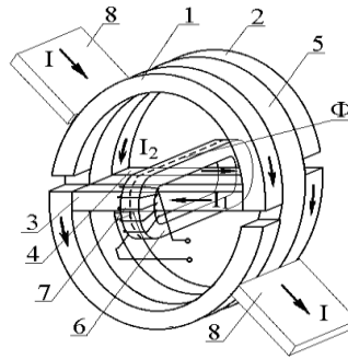
FIGURE 4. Axonometric view of the new transformer ferromagnetic current converter: 1, 2 – ring-shaped elements; 3, 4 – diametral connectors; 5 – dielectric layer; 6 – closed ferromagnetic core; 7 – secondary winding; 8 – current-receiving outputs
