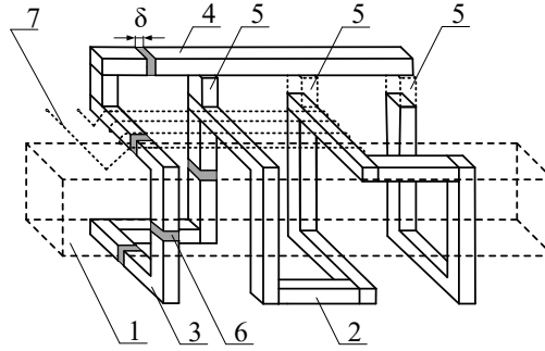
FIGURE 2. Variable-range ferromagnetic current transformer circuit
