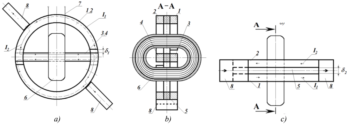
FIGURE 5. Structural diagrams of a ferromagnetic current transformer: a – view from the front, b – view from above
